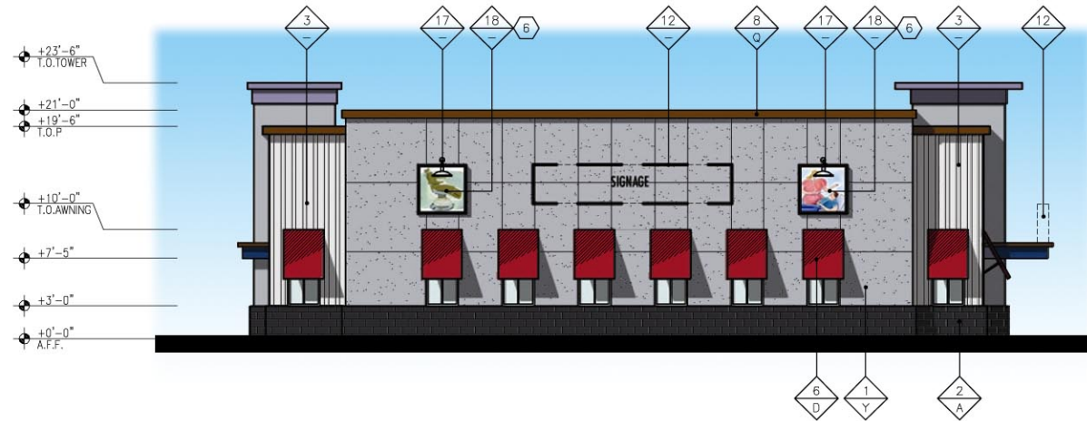
2. SOUTH ELEVATION
