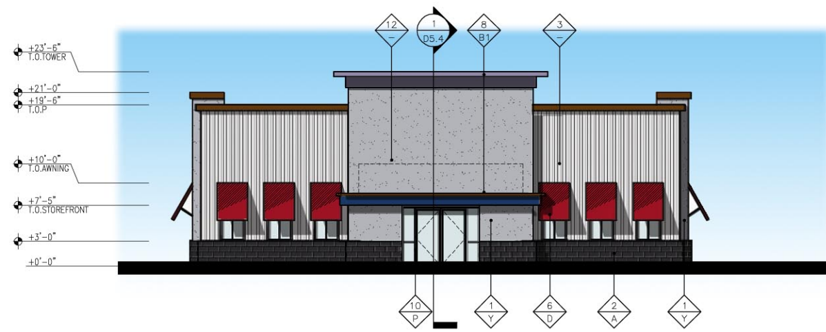
1. EAST ELEVATION
